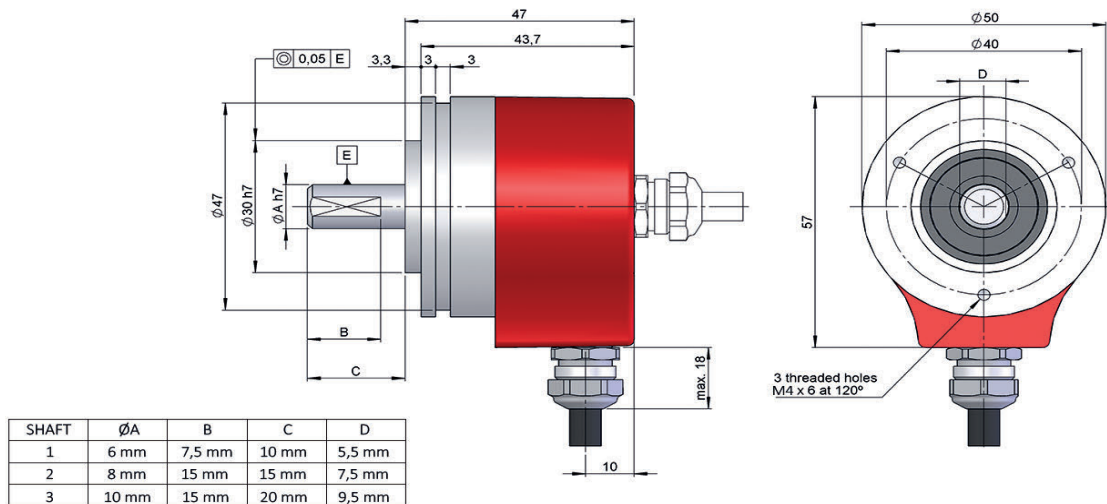
Drawing shaft type 3, connection type 1/4, without flange
